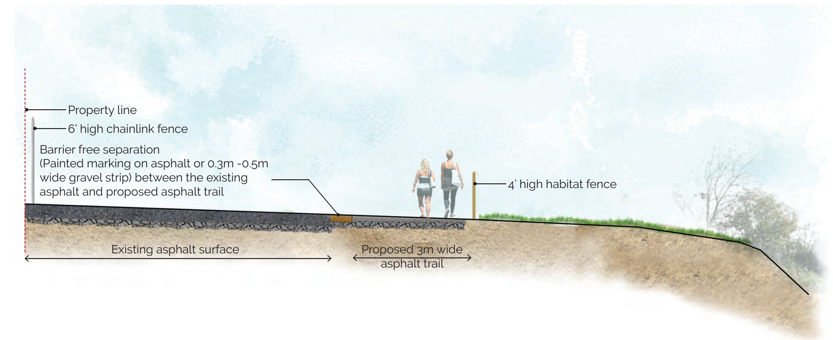
SECTION B-B
